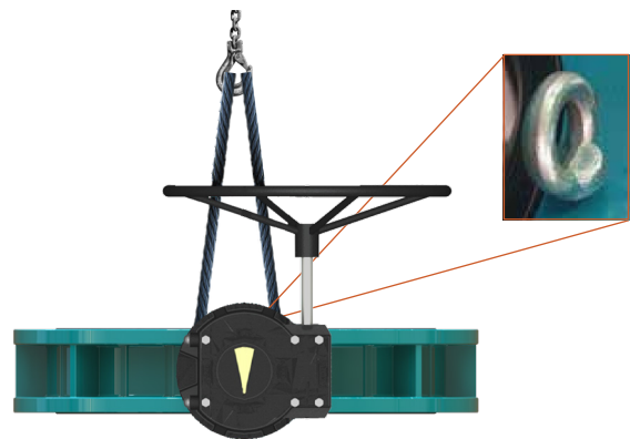
Horizontal installation
