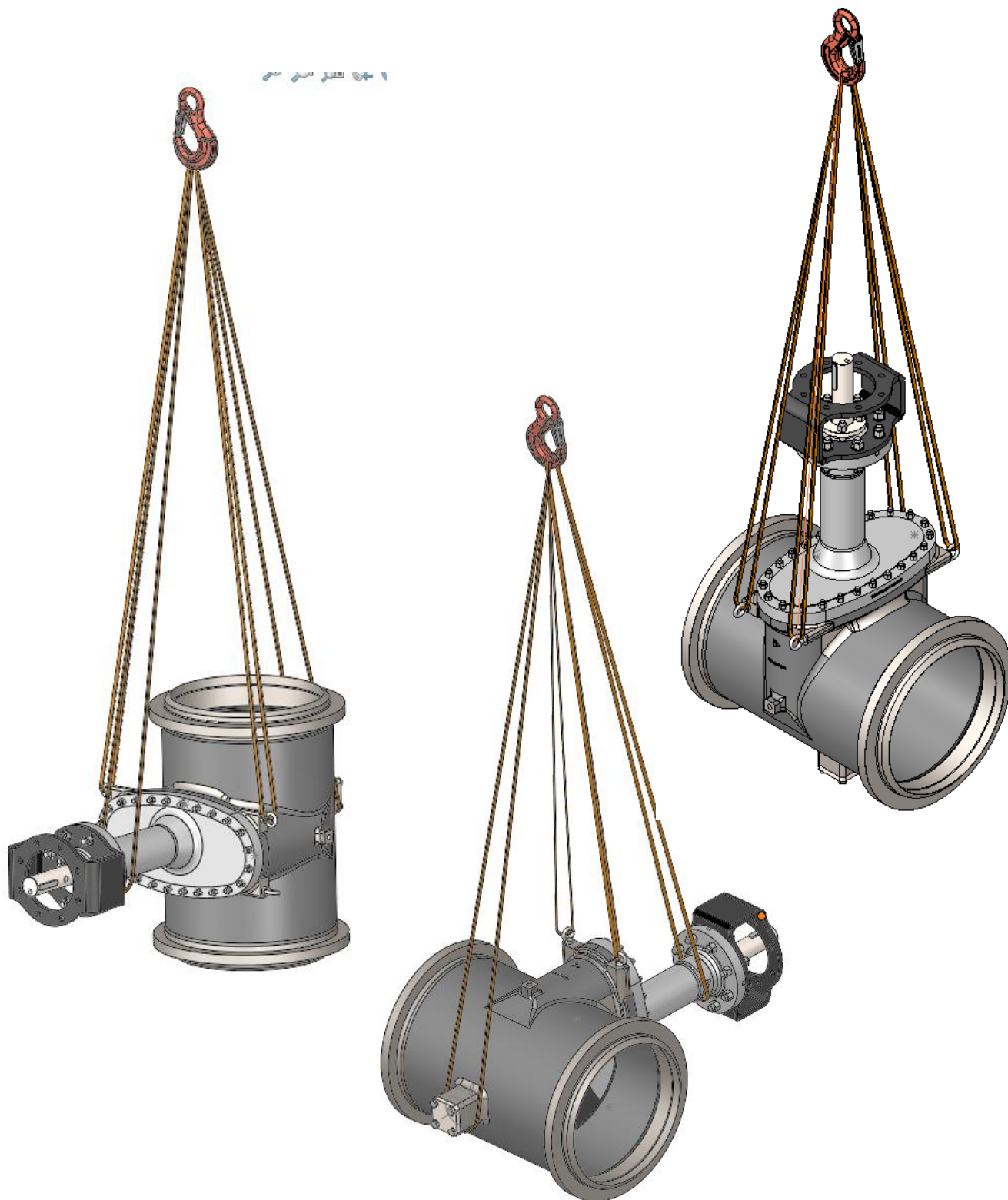
Fig 1 Handling
