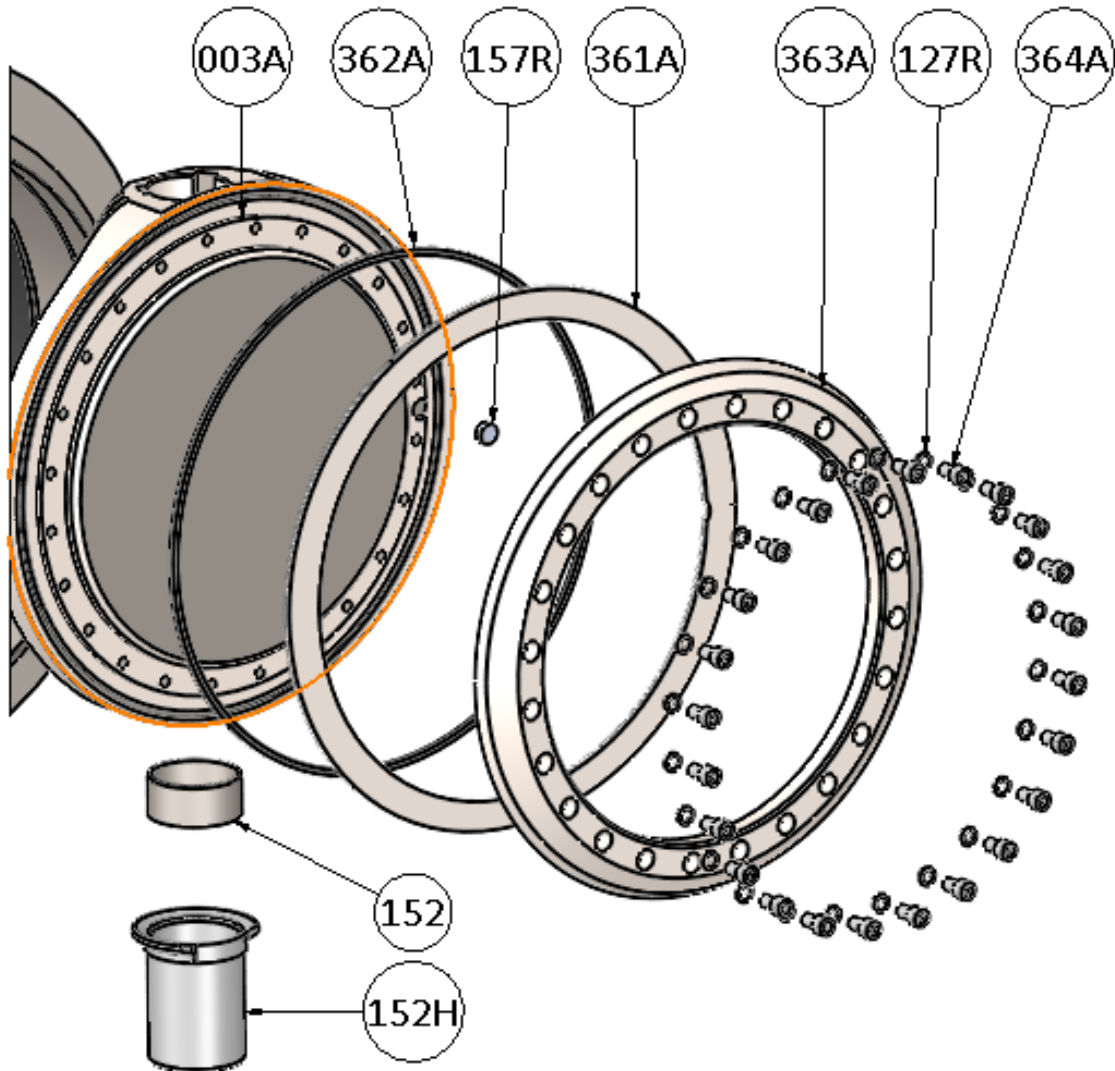
Fig 3 Seal ring maintenance
