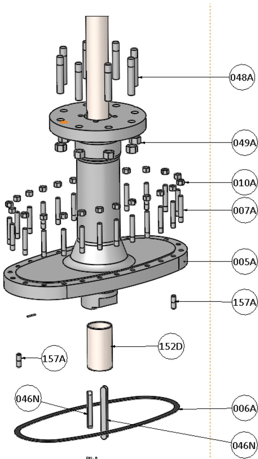
Fig. 4 Bonnet flange maintenance
