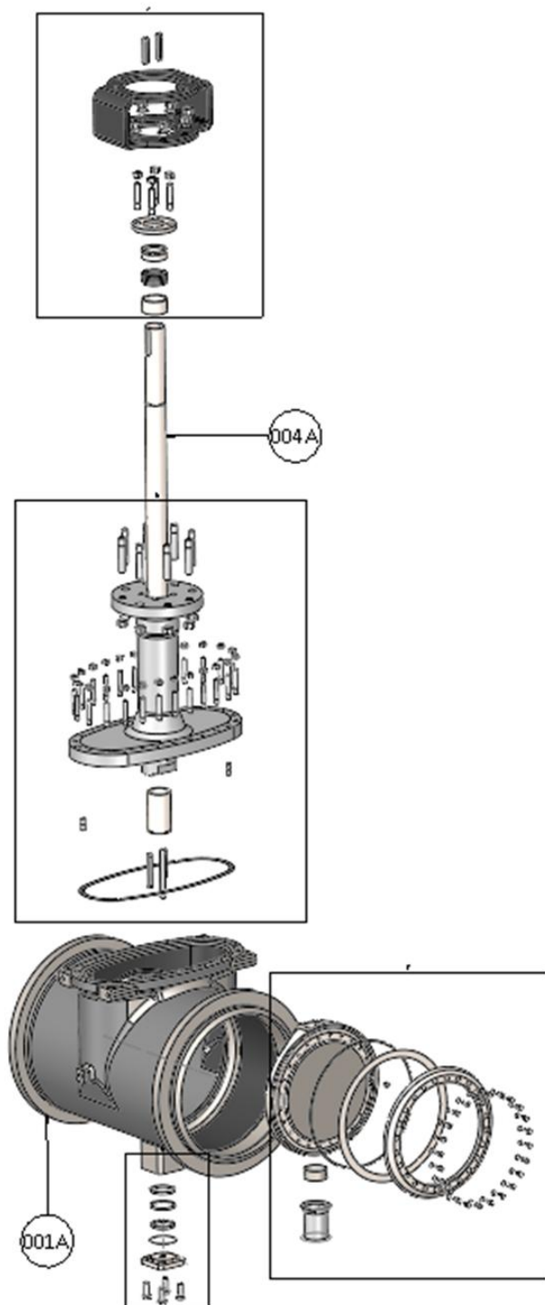
Fig 0 Exploded valve
