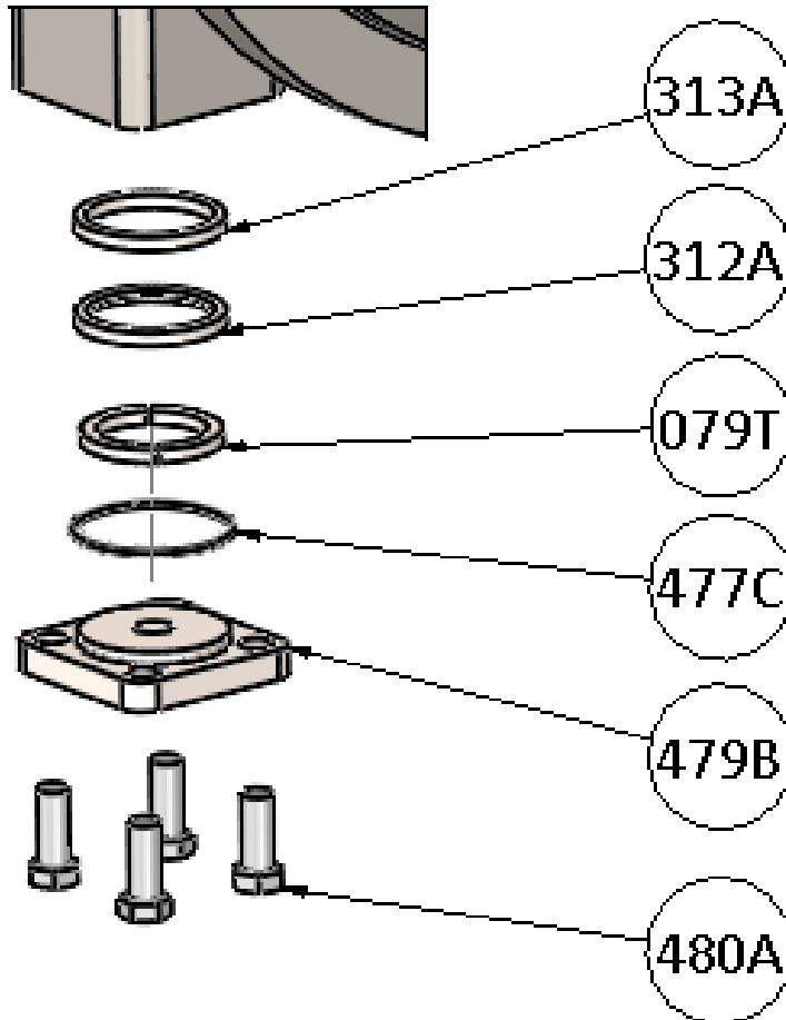
Fig 5 Bottom flange maintenance
