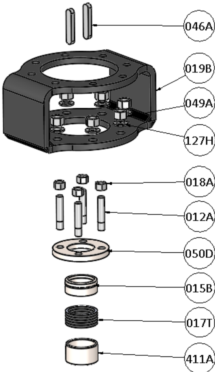
Fig 2 Packing maintenance
